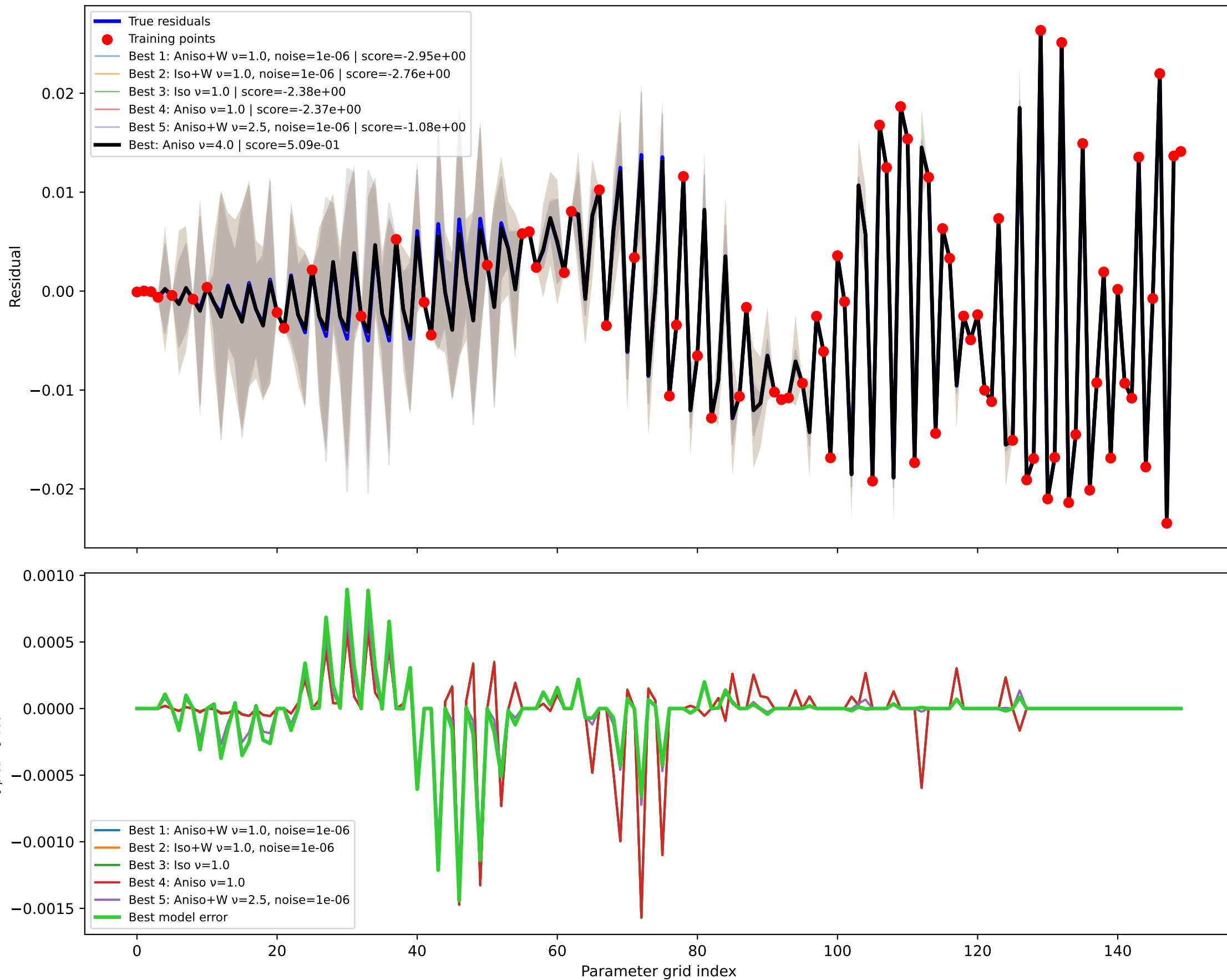
GPR kernel comparison node=34 RMSE=2.600e-04, train RMSE=1.533e-11
