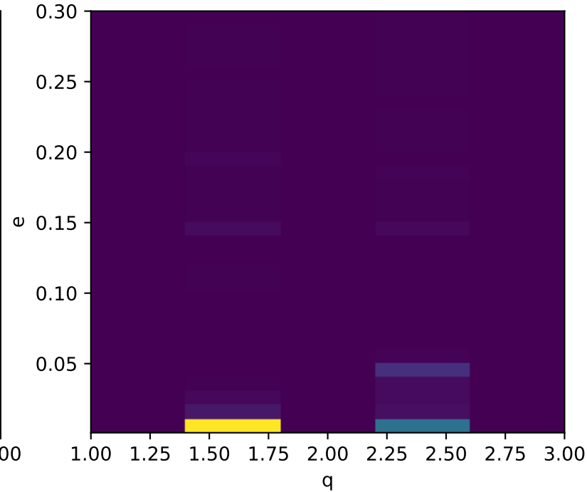
k=Aniso \nu=4.0
